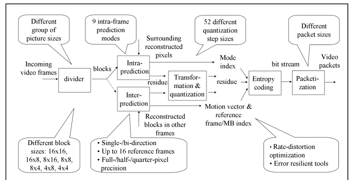
Fig. 1. Simplified diagram of AVC/H.264 encoder with different coding options and parameters
